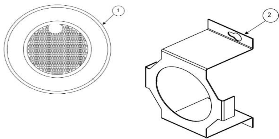
FIGURE 29: MEDIA TALKER SPEAKER AND BRACKET ASSY
