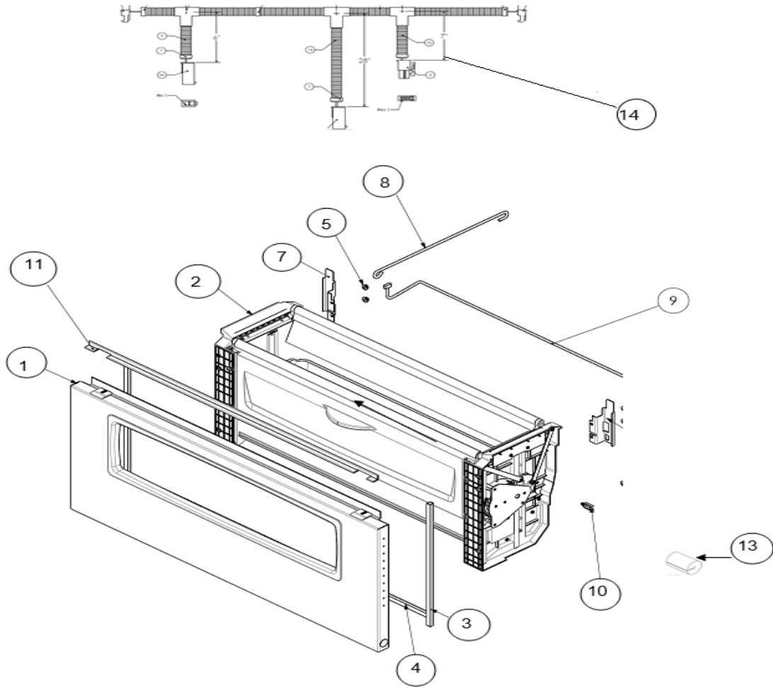
FIGURE 14: BIN & PANEL ASM COMBO
