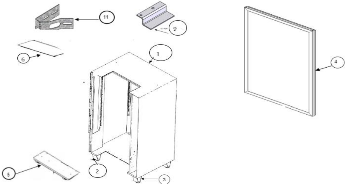
FIGURE 8: AMBIENT CABINET AND GLASS DOOR ASSEMBLY
