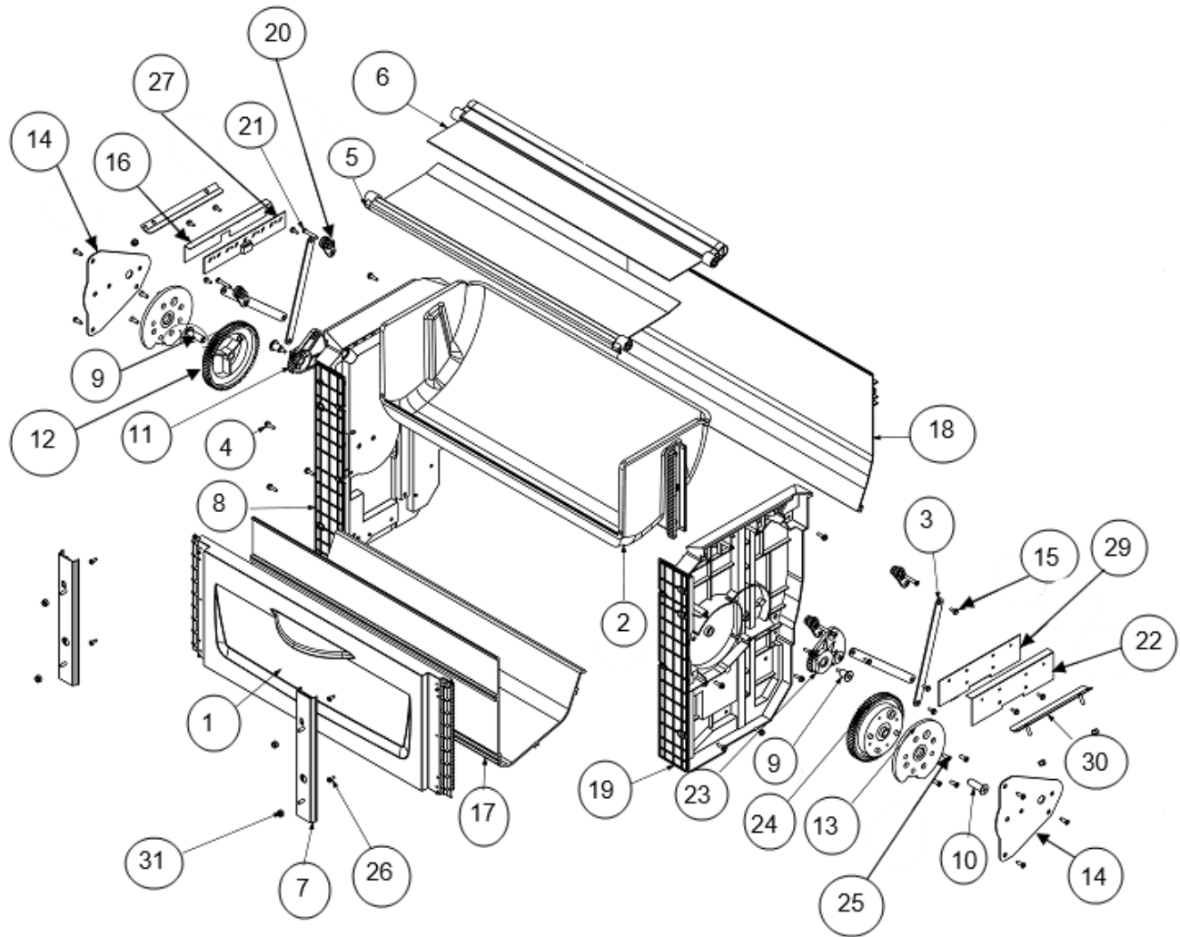
FIGURE 11: DEL BIN ASSEMBLY COMBO
