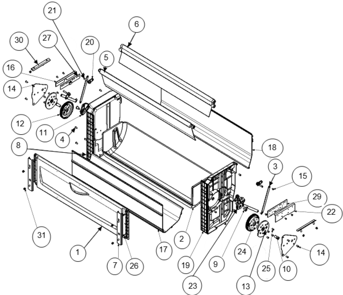
FIGURE 10: DEL BIN ASSEMBLY COMMON AMBIENT
