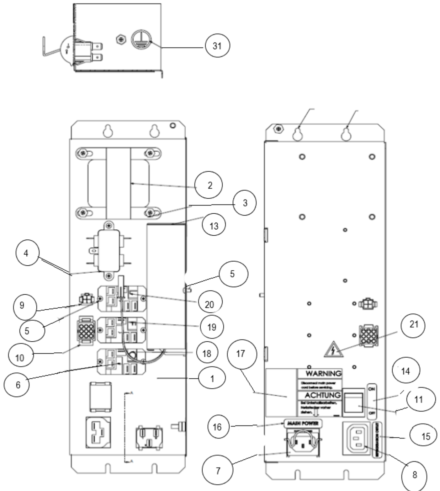
CRANE MERCHANDISING SYSTEMS FIGURE 26: ASSY AC BOX-230 VAC
