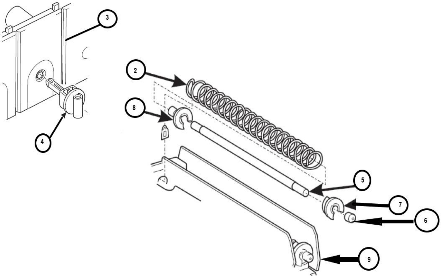
FIGURE 21: HALF CYCLE GUM & MINT SPIRAL ASSEMBLY
