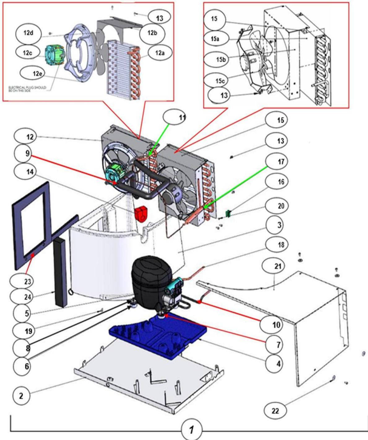
FIGURE 15: REFRIGERATION UNIT ASSEMBLY – COMBO
