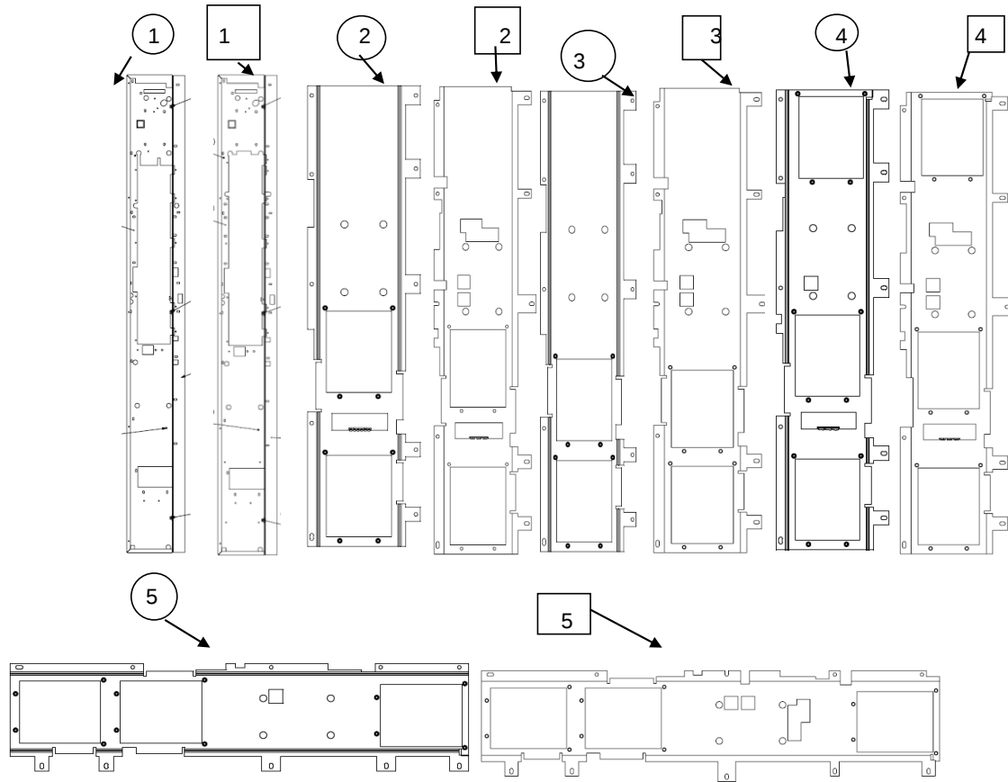
FIGURE 1A: ASSY, SERVICE DOOR BRACKETS
