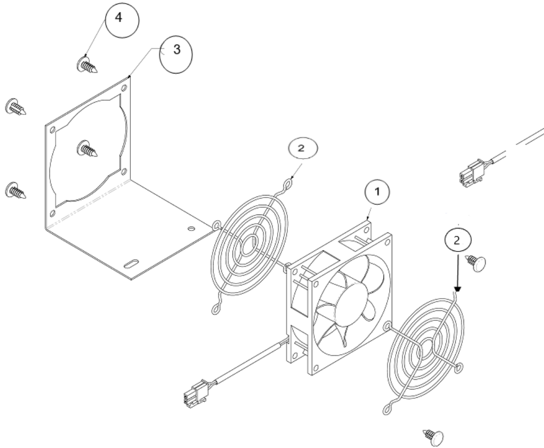
FIGURE 4: ASSY, MONETARY FAN MERCHANT AMBIENT
