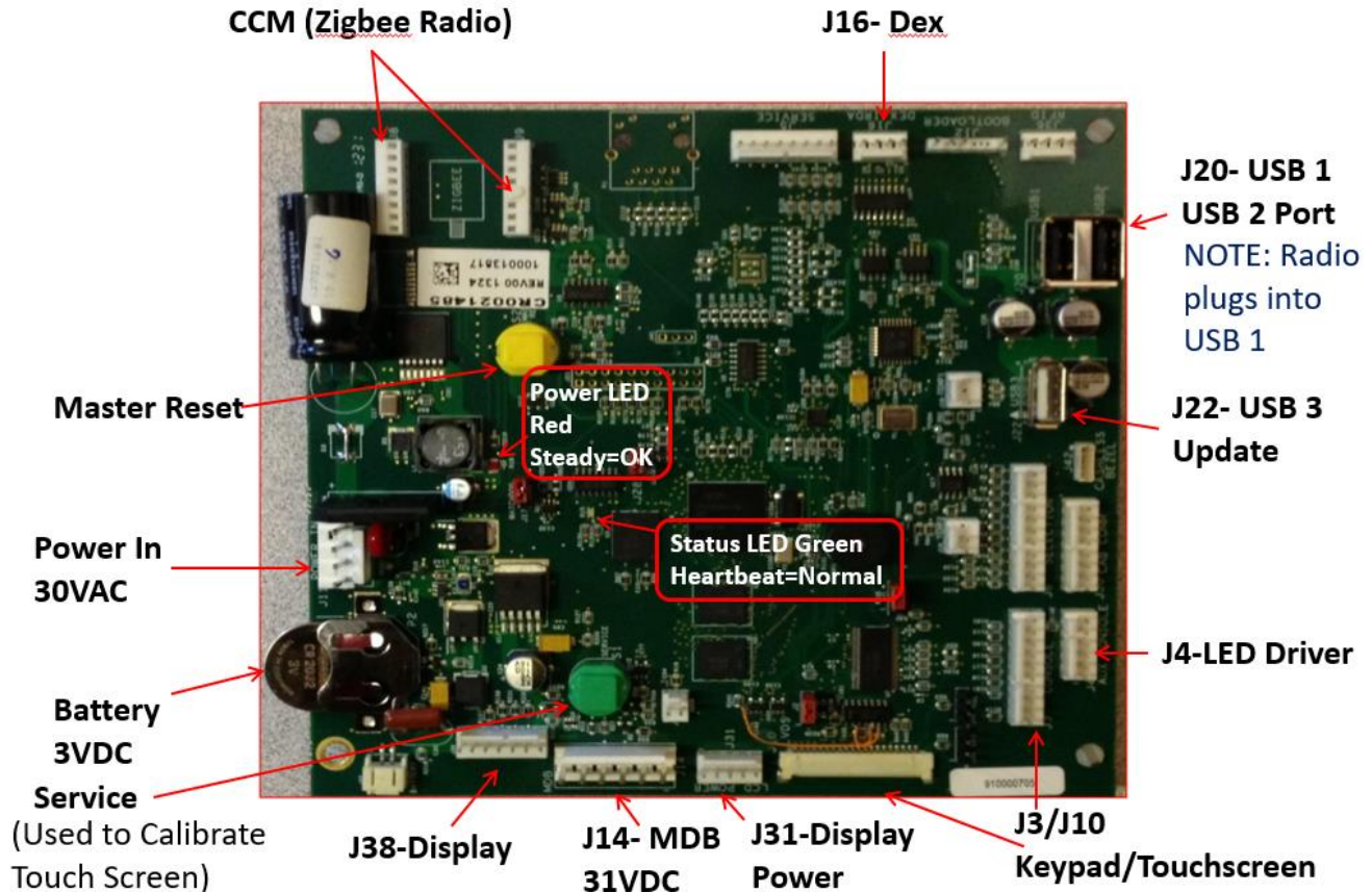
FIGURE 30A: Merchant Media (G-Board)
