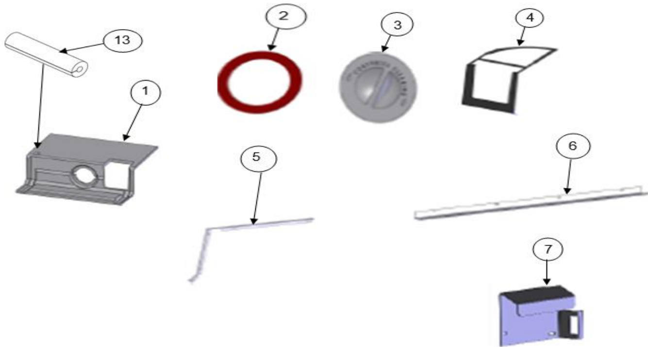
FIGURE 17: COMBO ADA BIN BARRIER
