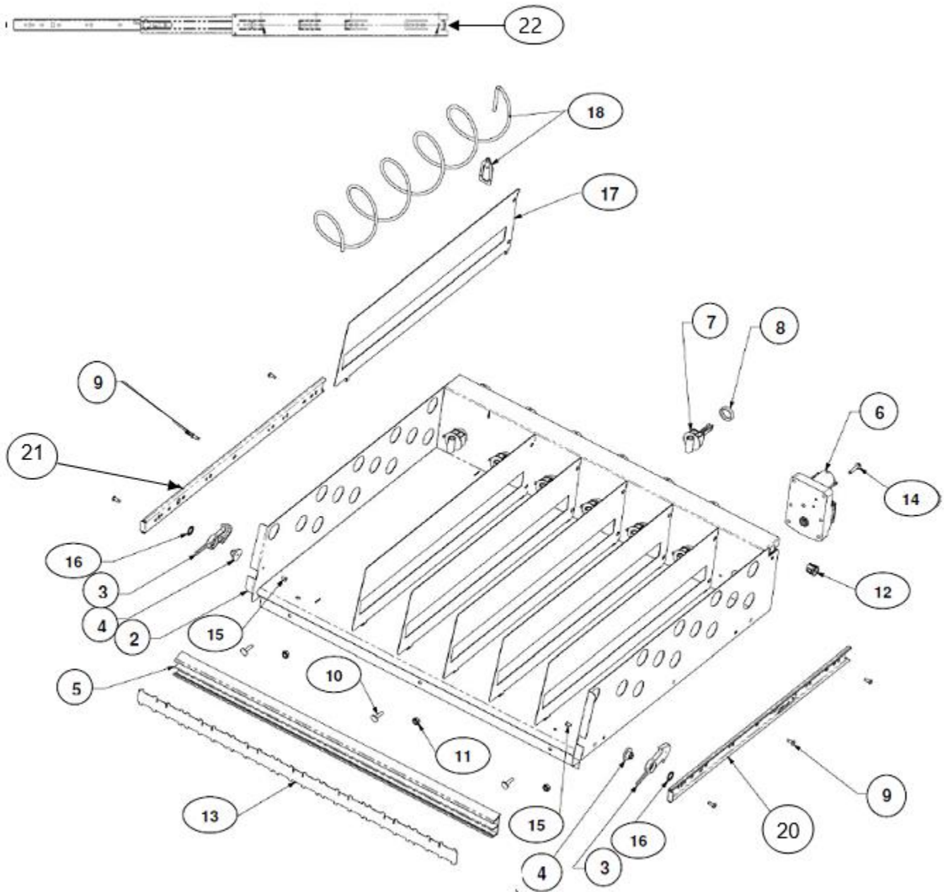
FIGURE 24: BOTTLE TRAY ASSEMBLY COMBO
