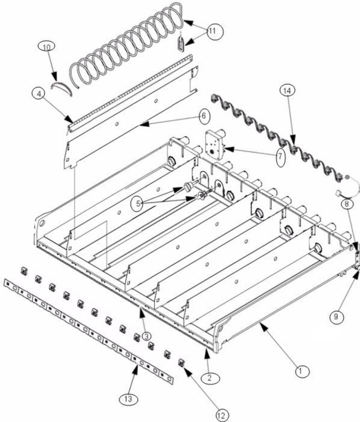
FIGURE 19: CANDY TRAY
