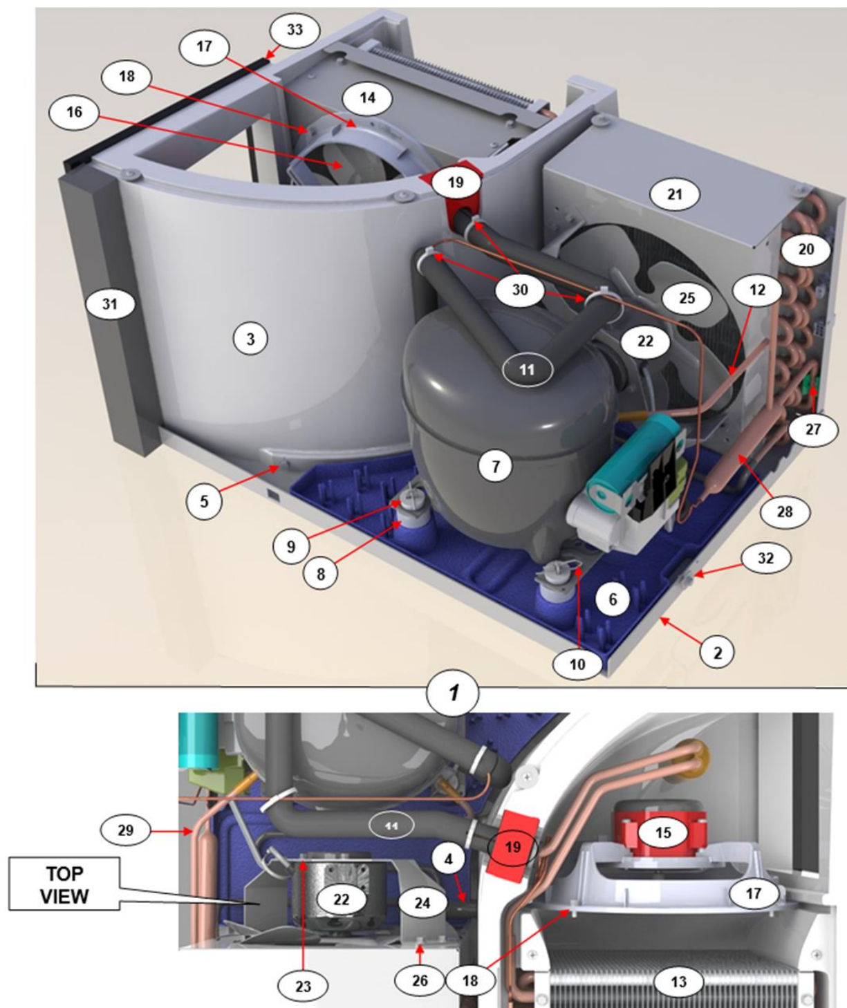
FIGURE 16: REFRIGERATION UNIT ASSEMBLY – 230VAC
